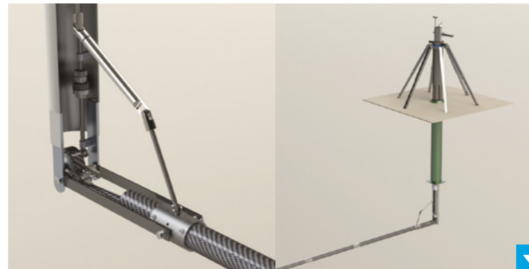
CLOSEUP OF HORIZONTAL ARM AND DRIVE MECHANISMS.
