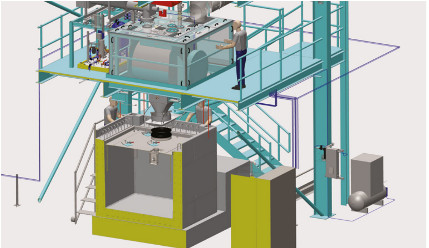
MAGNOX PRE-CONDITIONING LOT 4 CEMENTATION PLANT FOR HINKLEY A.
